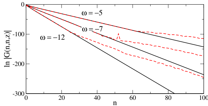
Figure 5. \ln |G(n, n, z)| versus n , for \omega = -5, -7, -12 , as given by the continued fractions (full black line) and direct integration (red dashed line). In all cases, \eta = 0.01 .
