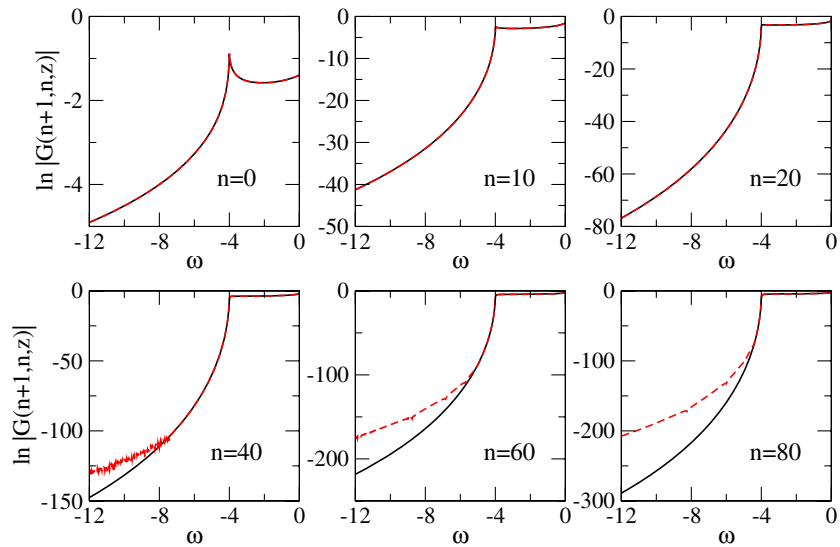
Figure 6. \ln |G(n + 1, n, z)| versus \omega , for n = 0, 10, 20, 40, 60, 80 , as given by the continued fractions (full black line) and direct integration (red dashed line). In all cases, \eta = 0.01 .
