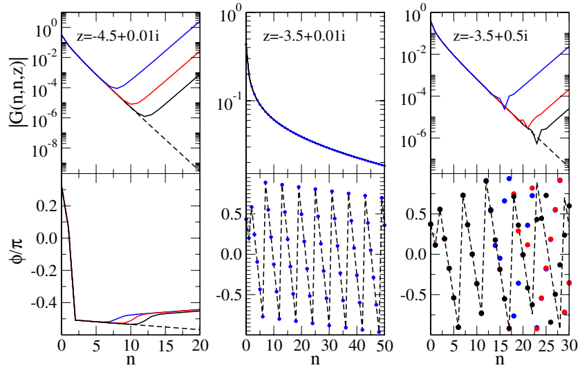
Figure 2. Top panels: absolute value |G(n, n, z)| versus n for three values of z . Bottom panels: phase of G(n, n, z) in units of \pi versus n , for the same values of z . The full lines correspond to the Morita solution, while the dashed ones are from direct numerical integration. The red/blue lines are the Morita solution where \delta A = 10^{-8} , respectively, 10^{-6} was added by hand to A(z) .
