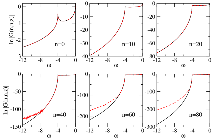
Figure 4. \ln |G(n, n, z)| versus \omega , for n = 0, 10, 20, 40, 60, 80 , as given by the continued fractions (full black line) and direct integration (red dashed line). In all cases, \eta = 0.01 .
