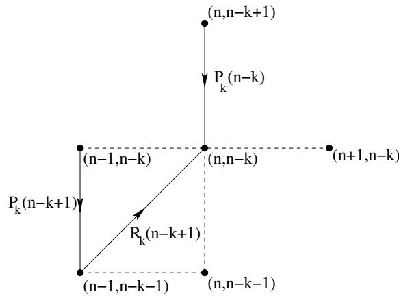
Figure 3. Ratios needed to express G(n, n-k+1, z) and G(n-1, n-k, z) in terms of G(n, n-k, z) (see the text for details).
