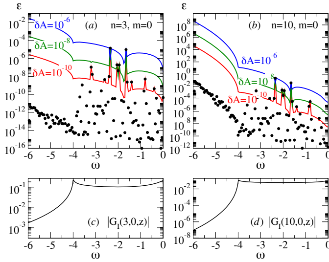
Figure 1. Relative error in the value of G(n, m, z) as estimated by the Morita scheme versus numerical integration (dots). The lines show the same quantity, when an absolute error of 10^{-10} , 10^{-8} respectively 10^{-6} is added by hand to the value of A(z) used in the Morita scheme. Here z = \omega + i\eta and \eta = 10^{-2} . Panel (a) corresponds to n = 3, m = 0 , while panel (b) to n = 10, m = 0 . Panels (c) and (d) show the value of |G(n, m, z)| as calculated by numerical integration.
